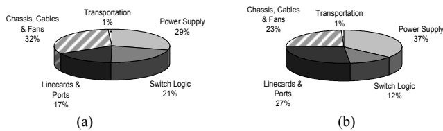
Figure 3. (a) Breakdown of energy use during manufacturing of a rack switch (energy to manufacture ~ 2.8 GJ-eq). (b) Breakdown of energy use during manufacturing of an aggregation switch (energy to manufacture ~ 4.7 GJ-eq).
