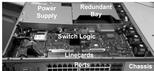
Figure 2. Typical 24-port 1U switch layout. We consider 48-port 1U switches that have similar layout in our study.
