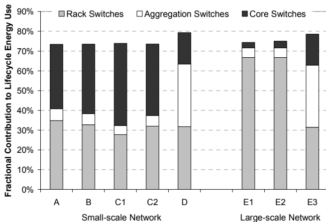
Figure 7. Relative contribution of different switch categories to the lifecycle energy use. (Balance is attributable to infrastructure energy use.) Note that for the fat-tree topologies (cases D and E3), the core and aggregation switching functions are performed by industry-standard commodity 1U switches.
