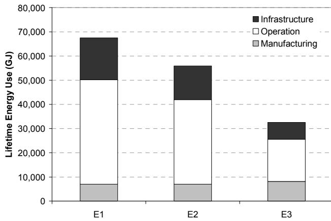
Figure 6. Lifetime energy use for some different topologies considered in Table 2, for a 1166-server network.
