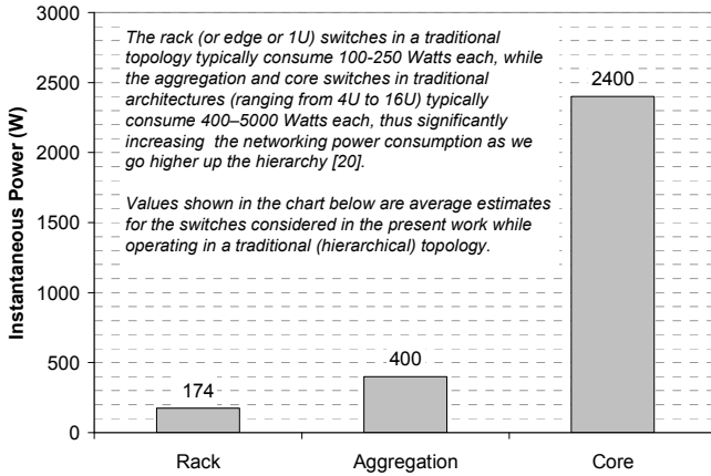
Figure 4. Instantaneous Power Use during operation of different switches.
