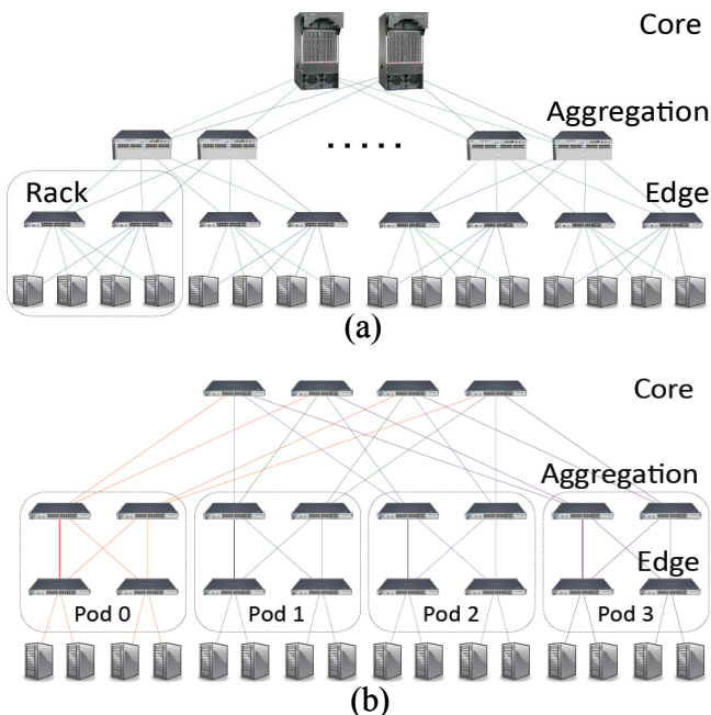
Figure 1. (a) A typical data center topology. Racks typically hold up to 40 “1U” servers and about two rack (edge) switches. (b) A fat-tree data center topology using only inexpensive commodity switches for the same number of end hosts (servers) as the typical topology.
