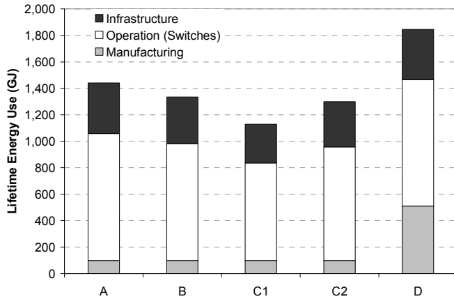
Figure 5. Lifetime energy use for some different topologies considered in Table 2, for a 292-server network.
